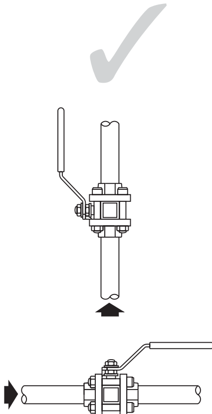
Fig. 3 Correct installation
