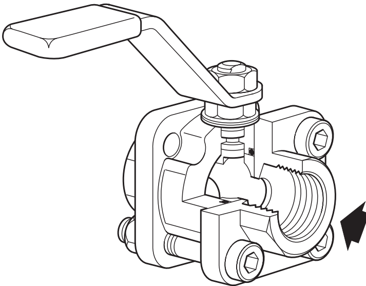
Fig. 1 M10HP ball valve
