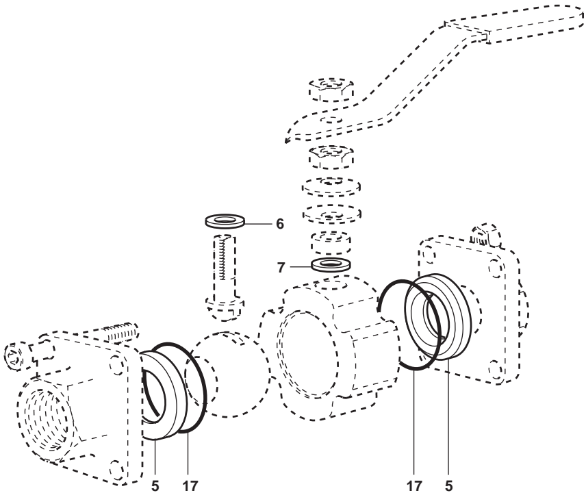
Fig. 5 M10HP screwed version shown
