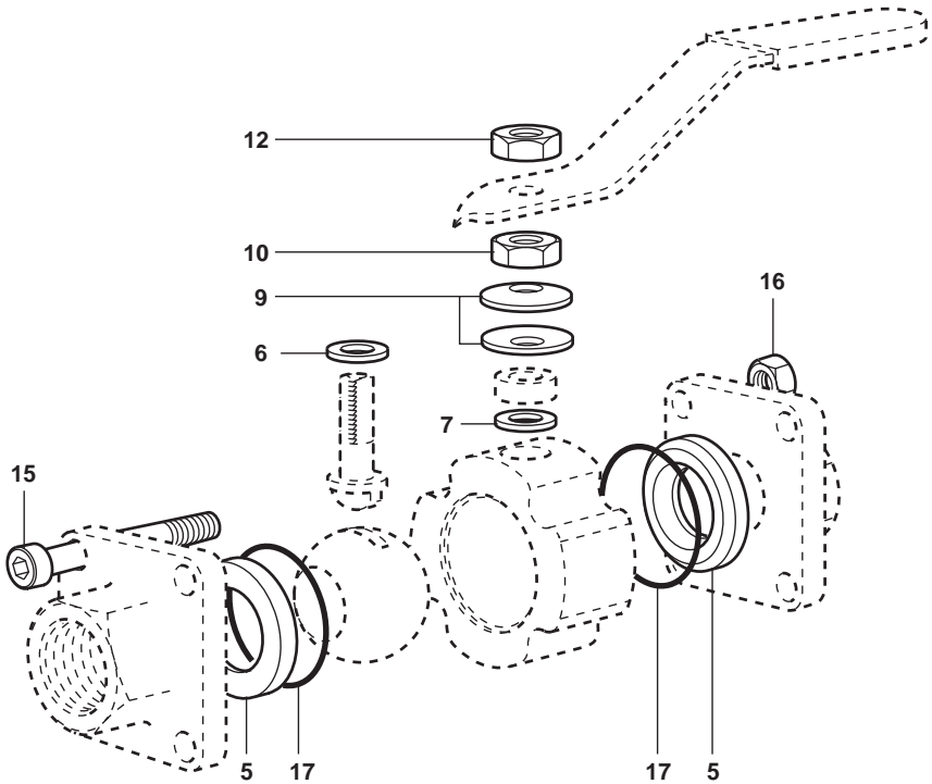
Fig. 4 M10HP screwed version shown
