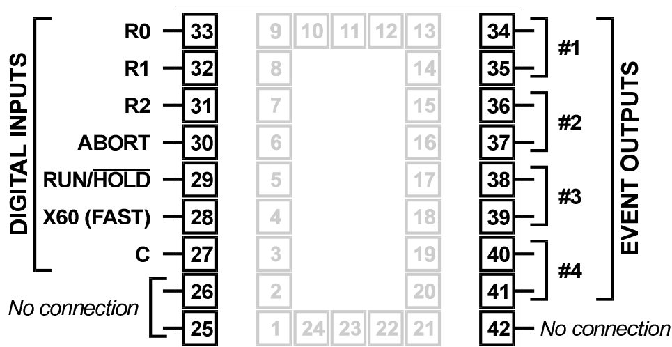
Figure 2-4 Rear Terminals
