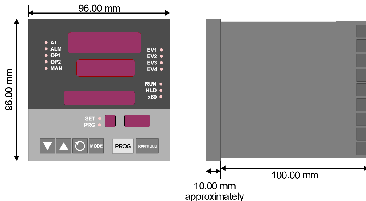
Figure 2-2 Principal Dimensions
