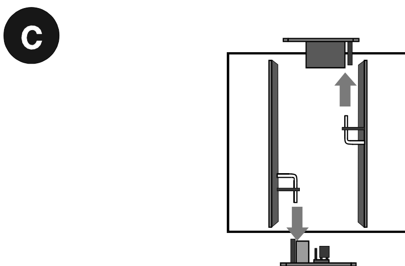
Figure 3-2 Removing the Output 2/Output 3 Option PCBs
