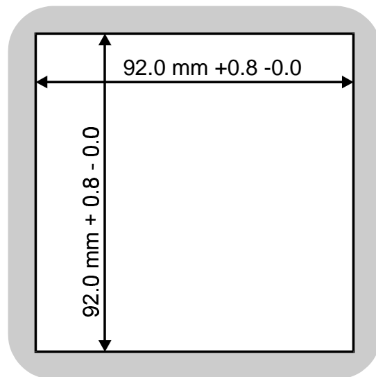
Figure 2-1 Cut-out Dimensions
